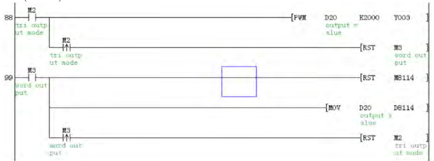
5) Use M2 for bit output, and use M3 for word output, in this project, it uses 2AD2DA-BD for analog output (4-20mA)
